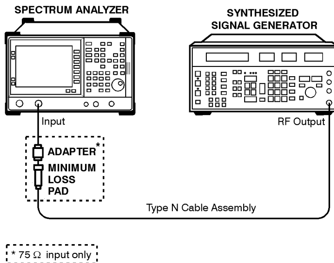
Residual FM Test Setup
