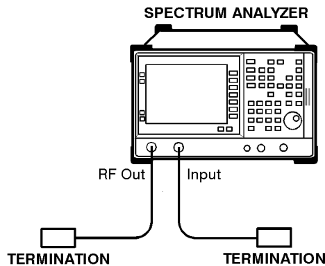
Tracking Generator Feedthrough Test Setup
