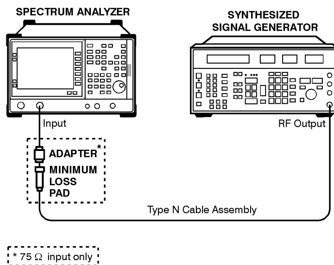
System Related Sidebands Test Setup
