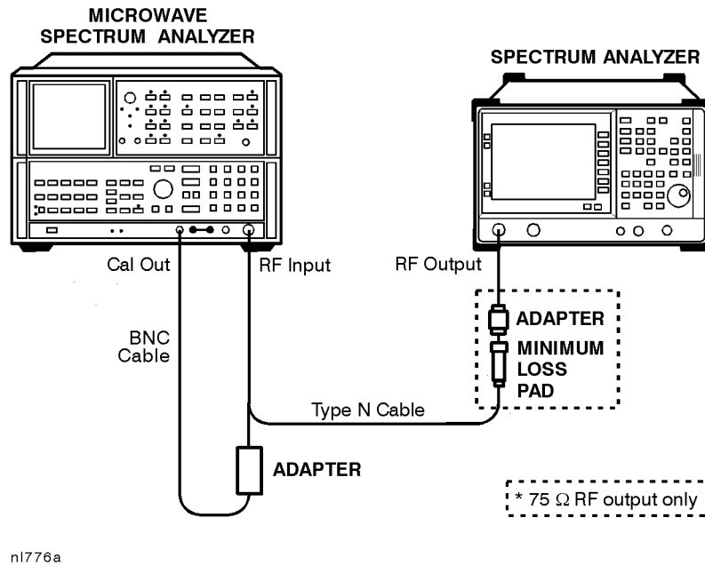
Figure 9-28 Non-Harmonic Spurious Outputs Test Setup
