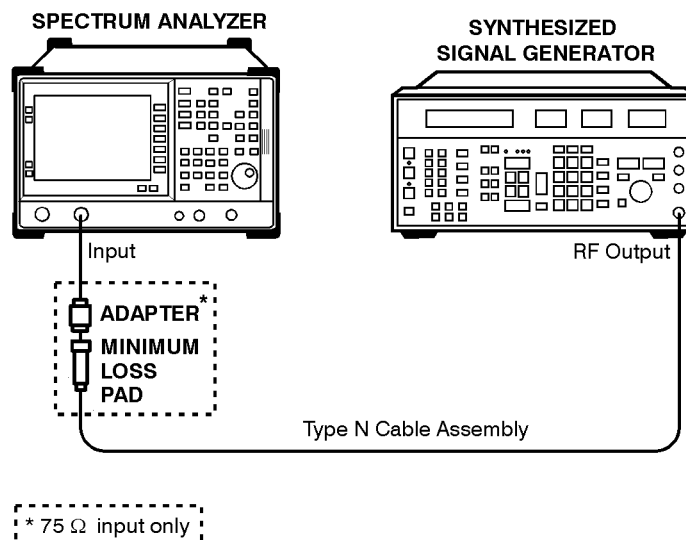
Noise Sidebands Test Setup
