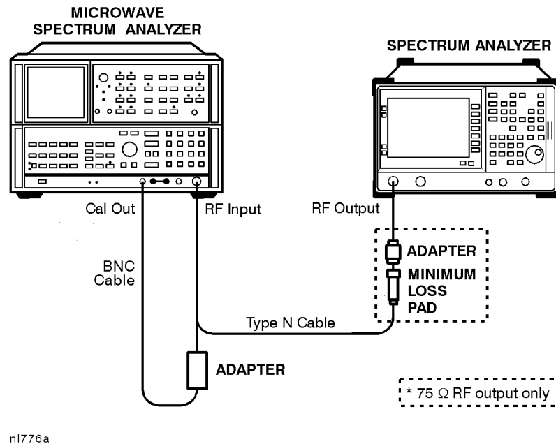
Harmonic Spurious Outputs Test Setup
